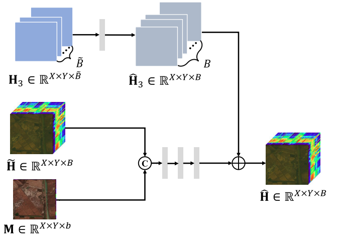
Fig. 5. Flowchart of the proposed SSRM. The upsampled LR-HSI and the HR-MSI are concatenated to extract residual information, which is then added to the band-aligned output of the third CMFM to produce the final fused result, enhancing spatial details while preserving spectral fidelity.
