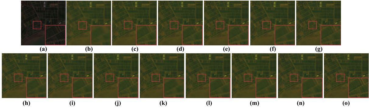
Fig. 10. Qualitative comparison of different methods on the YRE dataset. The results are shown by using the pseudocolor representation (R-60, G-29, and B-7). (a) MSI (Sentinel-2A). (b) HSI (Gaofen-5). (c) SSRNet. (d) ResTFNet. (e) MoG-DCN. (f) Fusformer. (g) DSPNet. (h) 3DT-Net. (i) DCTransformer. (j) PSTUN. (k) CYformer. (l) DMSN. (m) FusGAT. (n) DTUML. (o) Ours.
