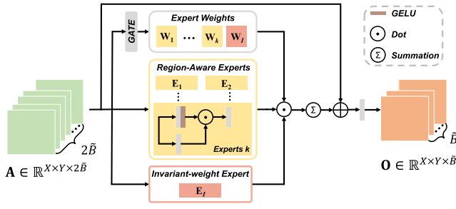
Fig. 3. Flowchart of the proposed region-aware MoE (RAMoE). The RAEs assign pixelwise adaptive weights, while the IWE applies a uniform weight across the entire image, thereby providing globally consistent guidance.
