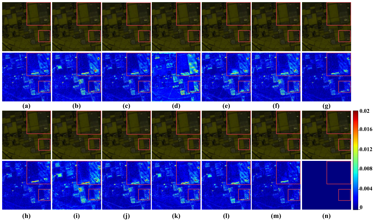
Fig. 8. Qualitative comparison of different methods on the Chikusei dataset. The first row shows the results using the pseudocolor representation (R-81, G-76, and B-2), and the second row is the corresponding error images. (a) SSRNet. (b) ResTFNet. (c) MoG-DCN. (d) DSPNet. (e) 3DT-Net. (f) DCTransformer. (g) PSTUN. (h) CYformer. (i) DMSN. (j) FusGAT. (k) DTUML. (l) DTUML. (m) Ours. (n) Reference.
