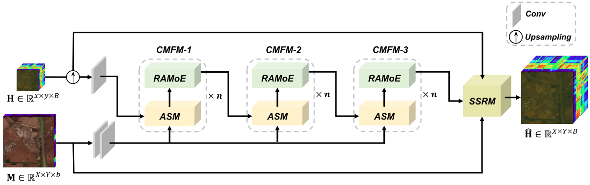
Fig. 1. Overview of the proposed RAMoE network architecture. The LR-HSI \mathbf{H} and the HR-MSI \mathbf{M} are jointly processed through three CMFMs. Each CMFM comprises n sequentially stacked blocks, where each block incorporates an ASM followed by the RAMoE. The fused features are finally refined by the SSRM to produce the reconstructed HR-HSI \hat{\mathbf{H}} .
