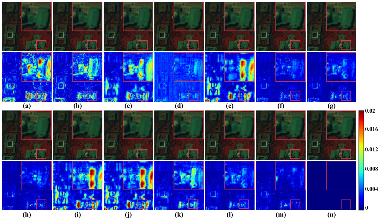
Fig. 7. Qualitative comparison of different methods on the WDCM dataset. The first row shows the results using the pseudocolor representation (R-65, G-30, and B-8), and the second row is the corresponding error images. (a) SSRNet. (b) ResTFNet. (c) MoG-DCN. (d) Fusformer. (e) DSPNet. (f) 3DT-Net. (g) DCTransformer. (h) PSTUN. (i) CYformer. (j) DMSN. (k) FusGAT. (l) DTUML. (m) Ours. (n) Reference.
