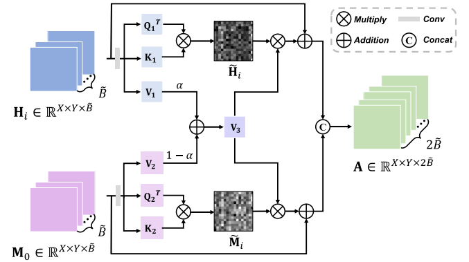
Fig. 2. Flowchart of the proposed ASM. The input \mathbf{H}_i denotes the iteratively fused feature at the i th stage, while \mathbf{M}_0 represents the initial feature extracted from the HR-MSI. A learnable scalar parameter \alpha is introduced to adaptively combine \mathbf{V}_1 and \mathbf{V}_2 , facilitating effective cross-modal interaction.
